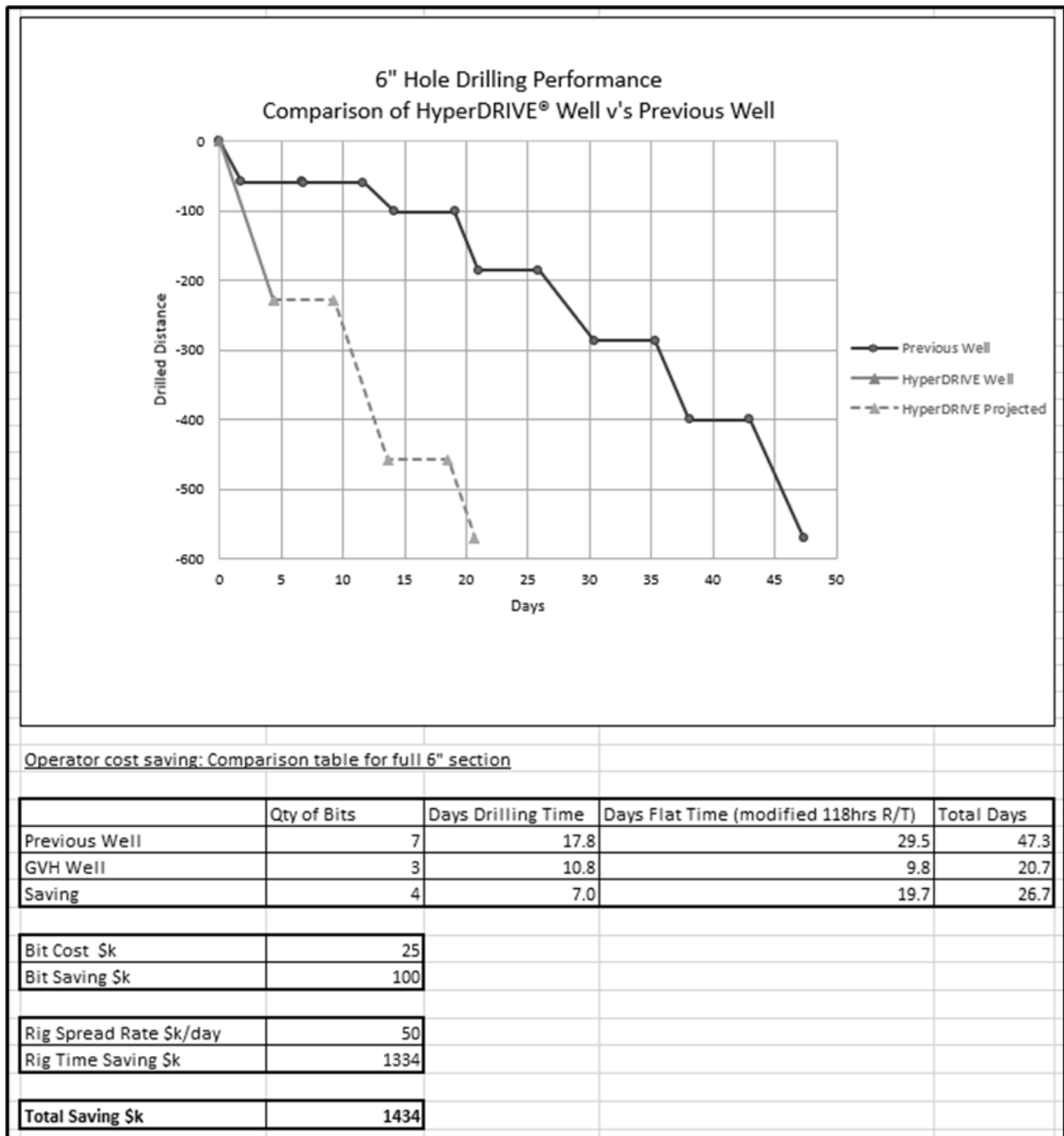
Figure 12: Time-Depth curve for offset well vs percussion-enhanced drilling.
