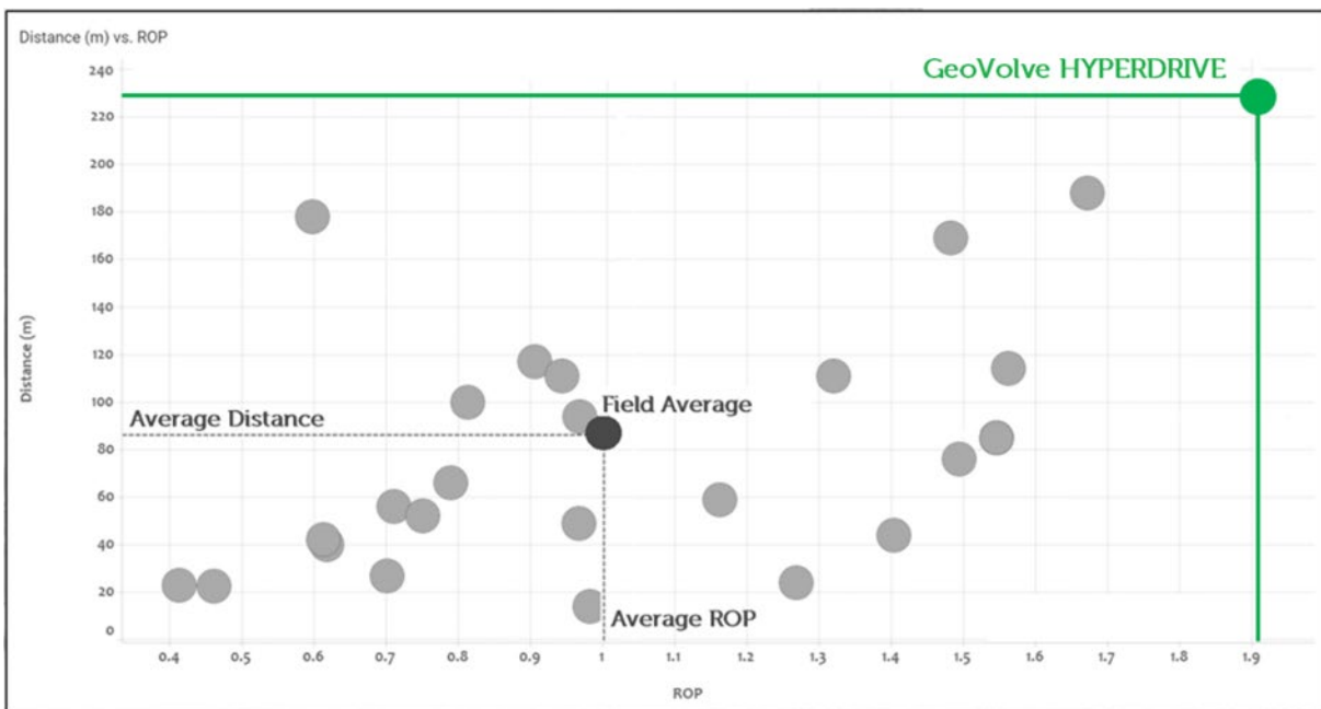
Figure 11: Distance vs ROP for all bit runs in basin, highlighting both average and percussion-enhanced drilling values.
