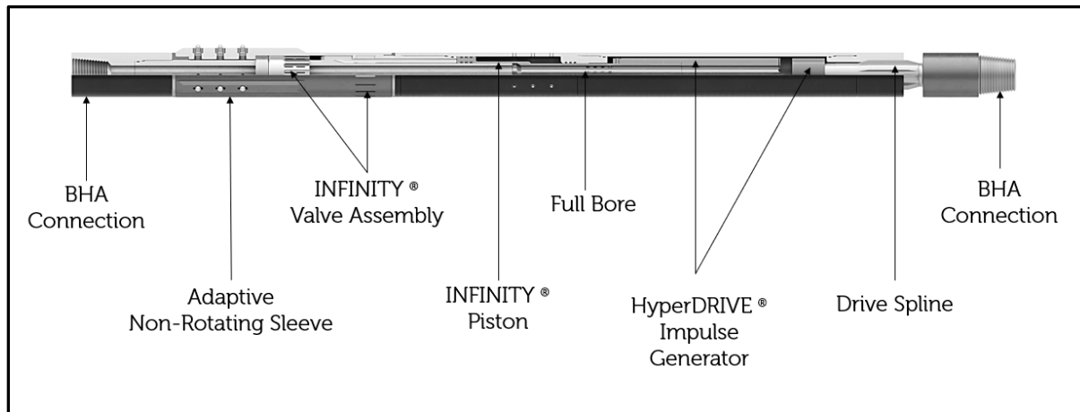
Figure 1. Layout of the Percussion-Enhanced Drilling System
