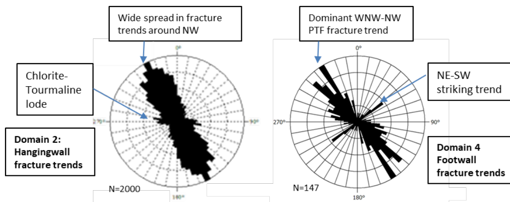
Figure 4: A comparison of the dominant fracture trends in Domains 2 and 4 (Foxford, 2019).
