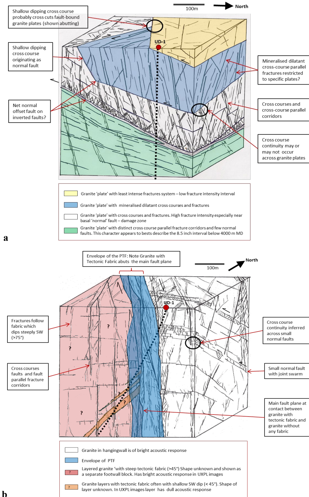
Figure 3: Preliminary schematic block diagrams of the structure encountered by well UD-1, characteristic of the a) hanging wall of the Porthtowan Fault at 1,750-3,400 m MD and b) 4,000-5,000 m MD (Foxford, 2019).
