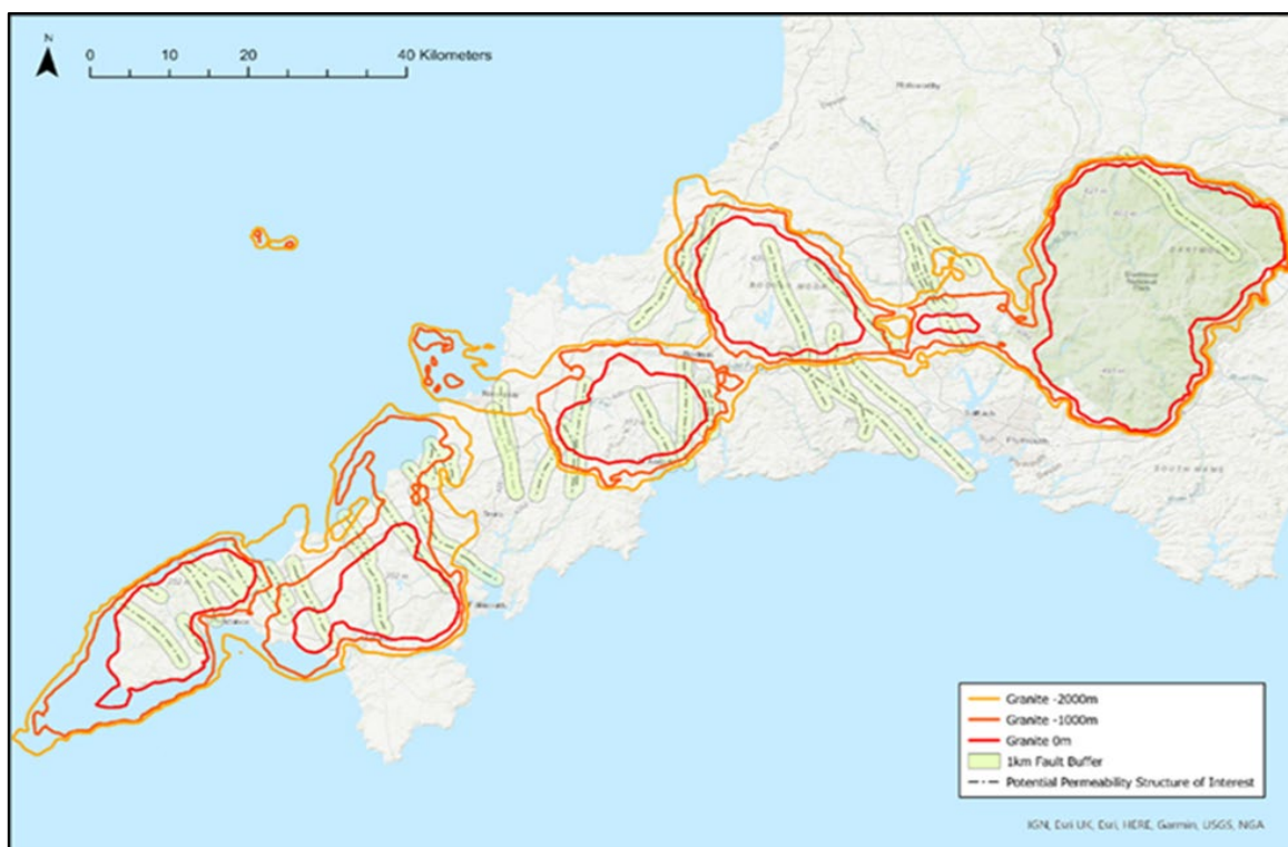
Figure 9: Depth to granite contours and permeability structures of interest across Southwest UK. Structures have been filtered out if they lie wholly outside the 2,000m depth to granite contour.
