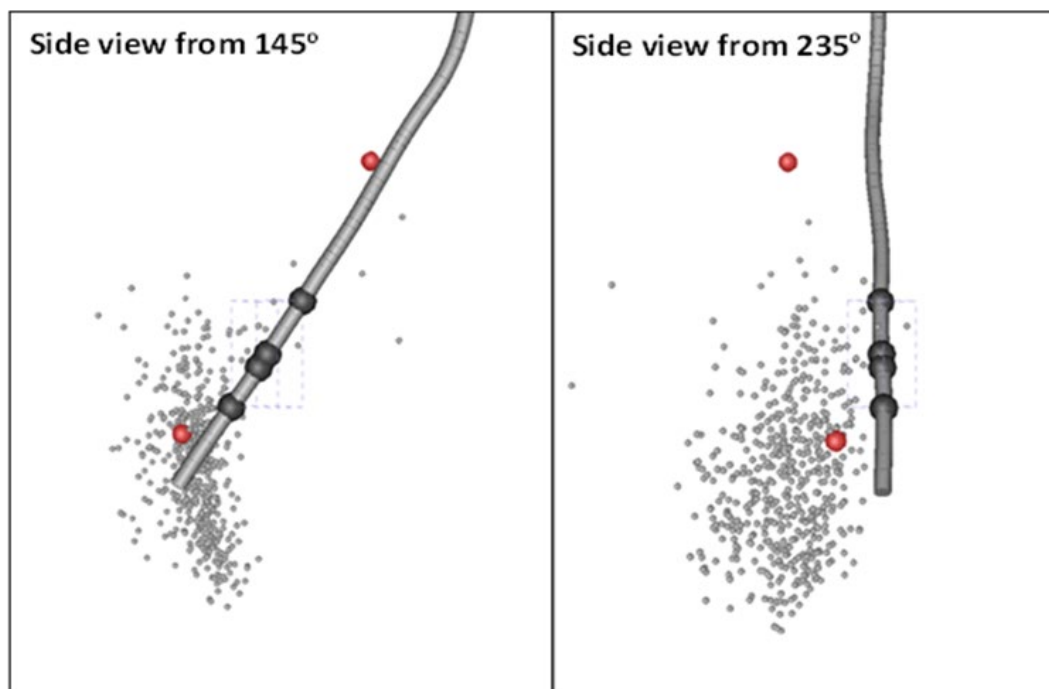
Figure 7: Location of the only two microseismic events which occurred during injection testing in July 2021 (red spheres), plotted against all previous seismic events during well testing at United Downs (grey spheres). The grey tube shows the well trajectory, with black sections indicating significant mud-loss zones during drilling. Images courtesy of Altcom Ltd.
