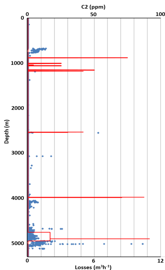
Figure 5: Drilling mud loss rates and C2 gas show abundance with depth through UD-1, highlighting the presence of permeable open fracture zones.
