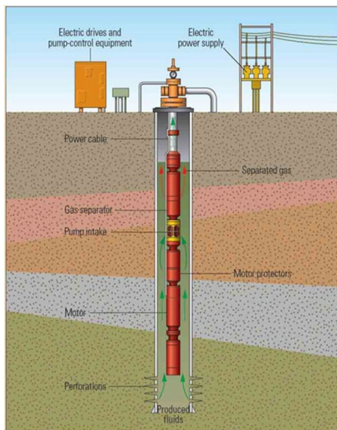
Figure 6: Schematic cross section of the key components of an electrical submersible pump in-situ. Image courtesy of Schlumberger.
