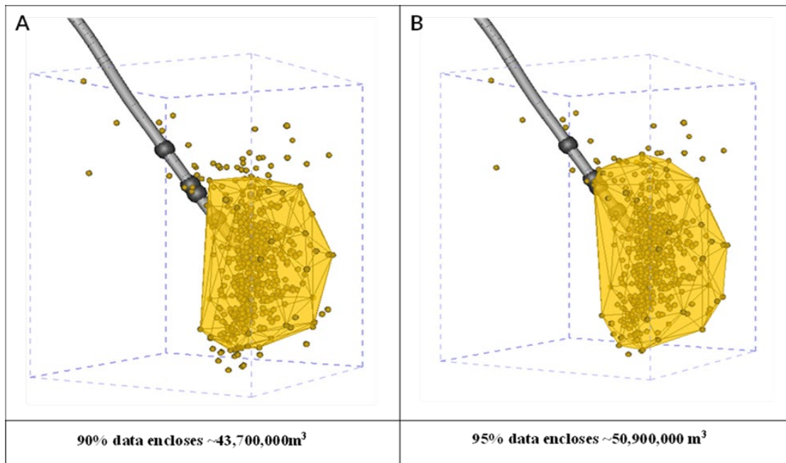
Figure 8: An estimate of stimulation volume after initial injection testing (up until February 2021) is provided by enclosing (A) 90% and (B) 95% of seismic events (closest to the centroid). Images courtesy of Altcom Ltd.
