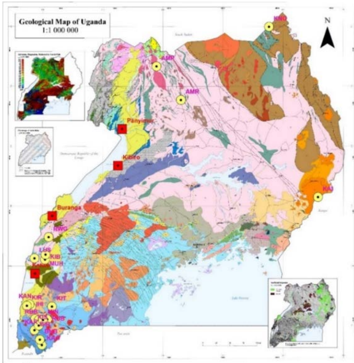
Figure 2: The geology of Uganda with the location of the geothermal areas. After Lehto et. al., 2014.
