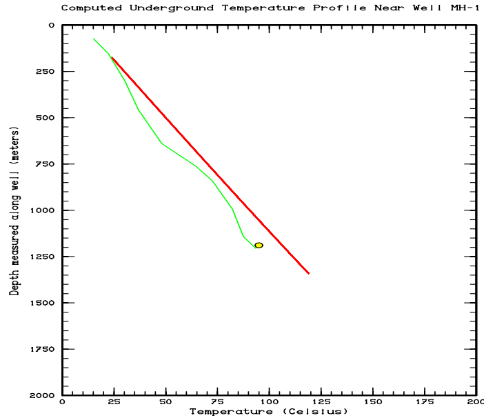
Figure 6: Comparison between computed (solid red line) and measured temperature profiles (solid green line and yellow circle) for well MH-1. No information is available concerning the shut-in time at which the temperature survey was taken.
