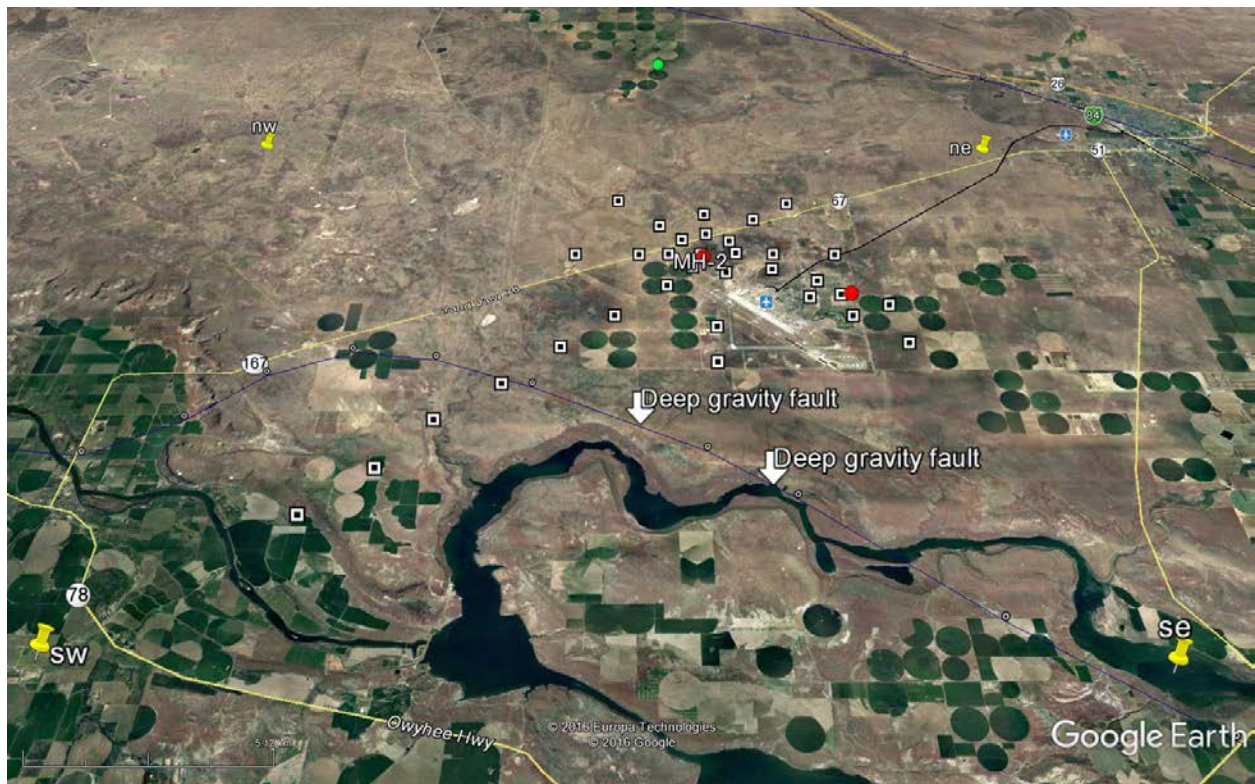
Figure 1: Mountain Home area showing the locations of boreholes MH-1 and MH-2 (red circles) and MT stations (white rectangles). The blue line (indicated by white arrows) passing to the south of MH-1 and MH-2 denotes a deep gravity fault. The NW (Lat: 43.1240, Long: -116.0780), NE (43.1211, -115.7707), SW (42.9439, -116.0807), and SE (42.9411, -115.7743) denote the four corners of the area (25 km by 20 km) used for the numerical model described below.
