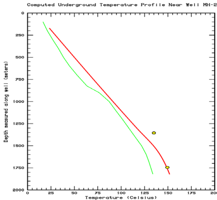
Figure 7: Comparison between computed (solid red line) and measured temperature profiles (solid green line) for well MH-2. The yellow circles are the measured flowing temperatures. Since the measured flowing temperatures are higher than the recorded shut-in temperatures (solid green line), it is almost certain that the shut-in survey does not represent the stable formation temperatures.
