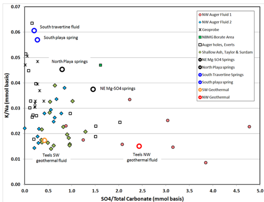
Figure 11: K/Na and \text{SO}_4 /total carbonate ratios of groundwater and spring samples from within and adjacent to Teels Marsh. Geothermal fluids northwest of the playa (open red circle) have solute ratios similar to that of auger brines in the northwest corner of the playa (small red circles). Auger fluids 1 and 2 are from Dajin's second auger sampling campaign. Shallow ash samples are from Taylor and Surdam (1981) and Everts samples from Everts (1969). North playa, Mg-SO 4 , and South travertine fluids from Smith and Drever (1976). Teels geothermal fluid and South playa spring samples from Geothermal Development Associates (unpublished data). Figure from Coolbaugh and Hickson, 2017.
