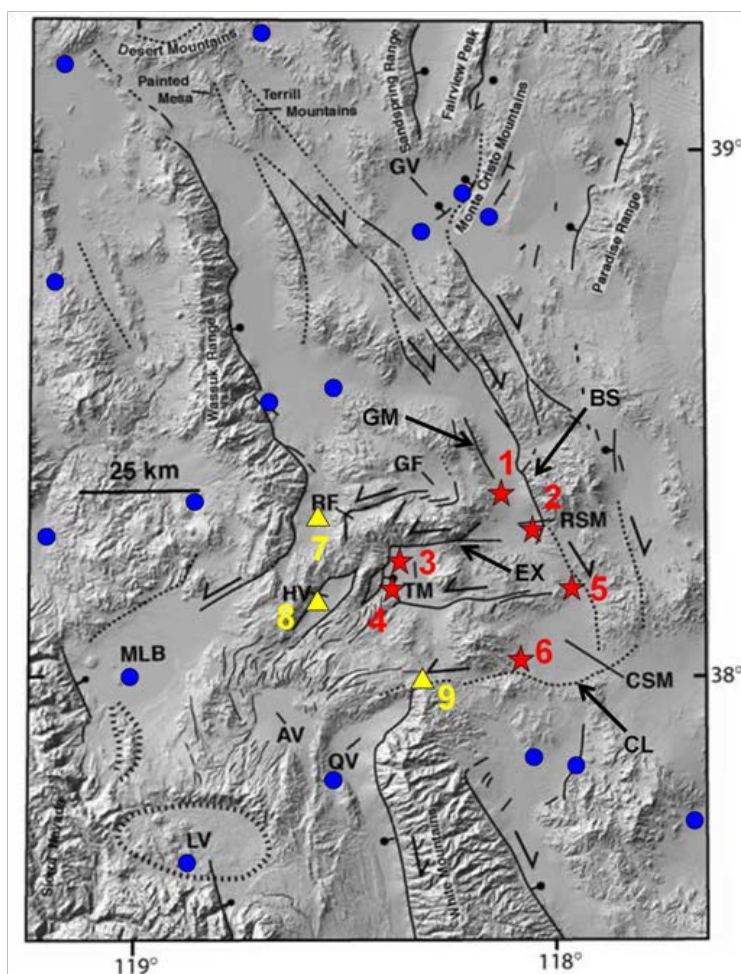
Figure 7: Quaternary faults and geothermal systems in the Mina Deflection. The physical extent of the Mina Deflection encompasses the geothermal areas: 1 = Sodaville, 2 = Rhodes Marsh, 3 & 4 = North & south Teels Marsh, 5 = Redlich, 6 = SW Columbus Marsh; and thermal wells 7, 8, and 9 at Whiskey Flat, Huntoon Valley, and NE of Queen Valley, respectively. RSM = Rhodes Salt Marsh, TM = Teels Marsh, CSM = Columbus Salt Marsh, GF = Garfield Flat, HV = Huntoon Valley, RF = Rattlesnake Flat, MLB = Mono Lake Basin, LV = Long Valley caldera, AV = Adobe Valley, QV = Queen Valley, GV = Gabbs Valley, EX = Excelsior Mountain fault, GM = Gumdrop Hills fault, CL = Coaldale fault, BS = Benton Springs fault. Blue circles are geothermal systems outside the Mina Deflection with measured or estimated temperatures >70°C. Taken from Coolbaugh et al. (2013) and originally adapted from Wesnousky (2005).
