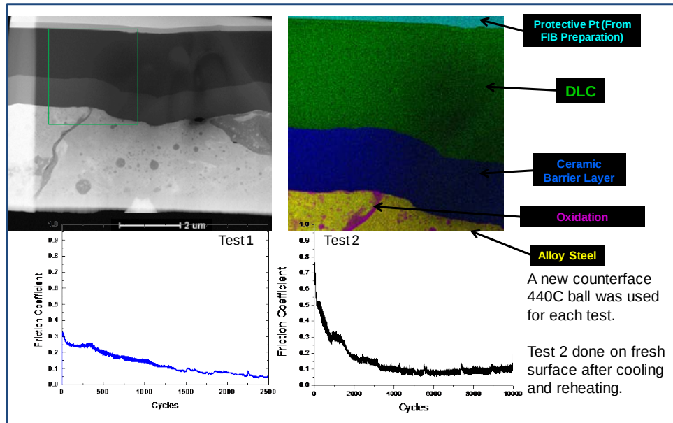
Figure 7. Results for DLC nanocomposite on ceramic layer
