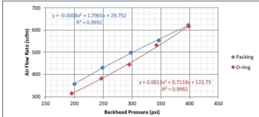
Figure 10. Flow rate vs. backhead pressure for preliminary baseline design
