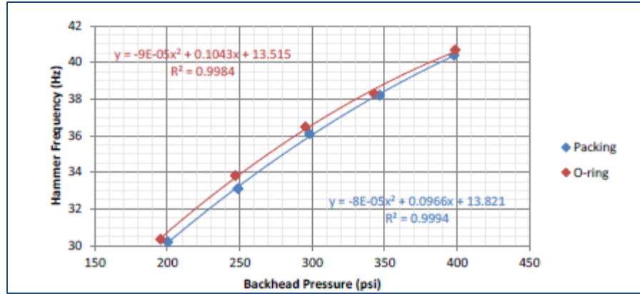
Figure 12. Hammer frequency vs. backhead pressure for preliminary baseline design
