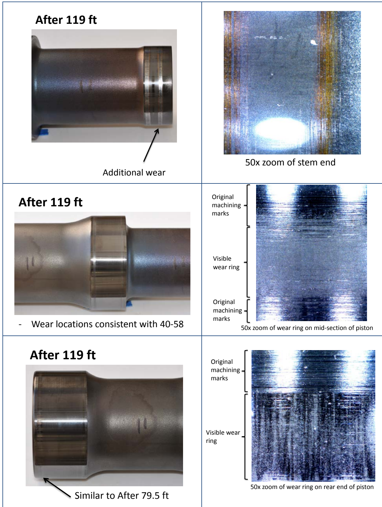
Figure 31. LT piston with DLC inspection results after 119 ft.
