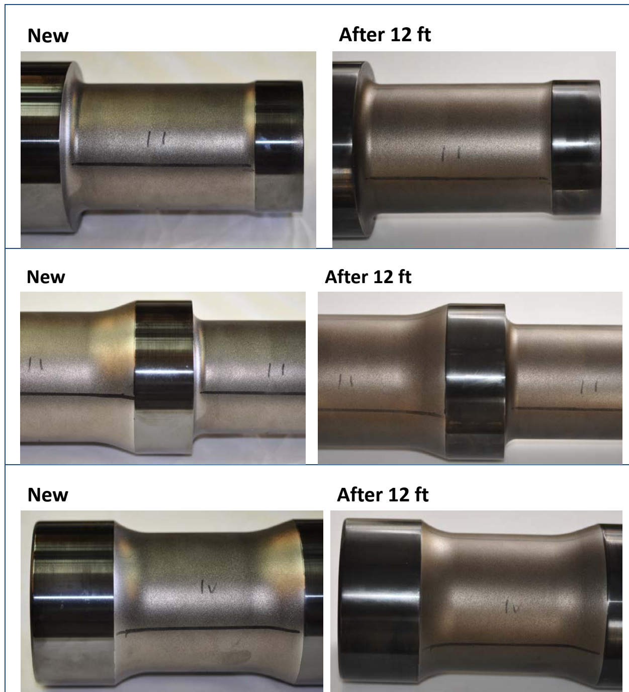
Figure 30. LT piston with DLC coating applied (inspection new and after 12 ft)
