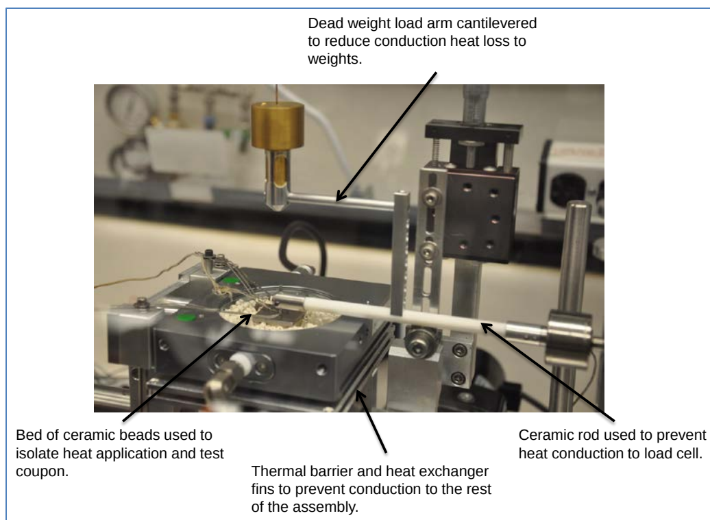
Figure 5. High-temperature tribometer for friction and wear used to characterize friction on surfaces
