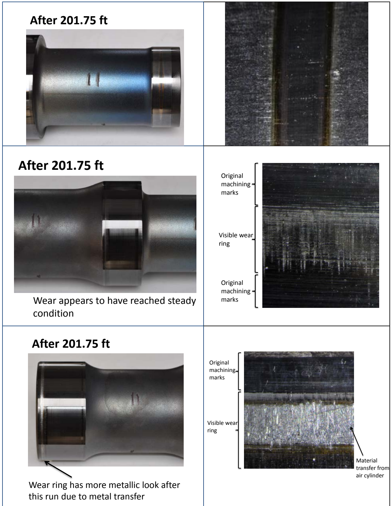
Figure 34. LT piston with DLC inspection after 201.75 ft.
