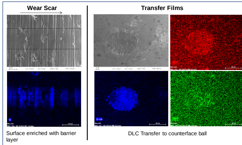
Figure 8. Wear scars and transfer films of tested samples
