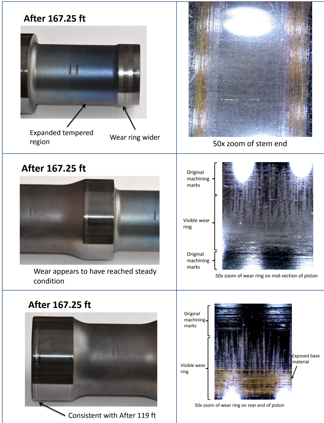
Figure 33. LT piston with DLC inspection after 167.25 ft.
