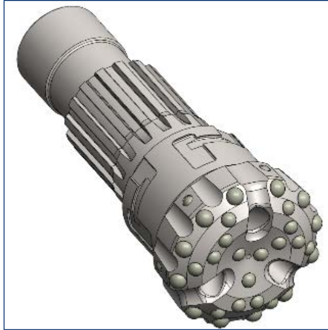
Figure 2. Hammer bit illustration showing buttons within the bit body
