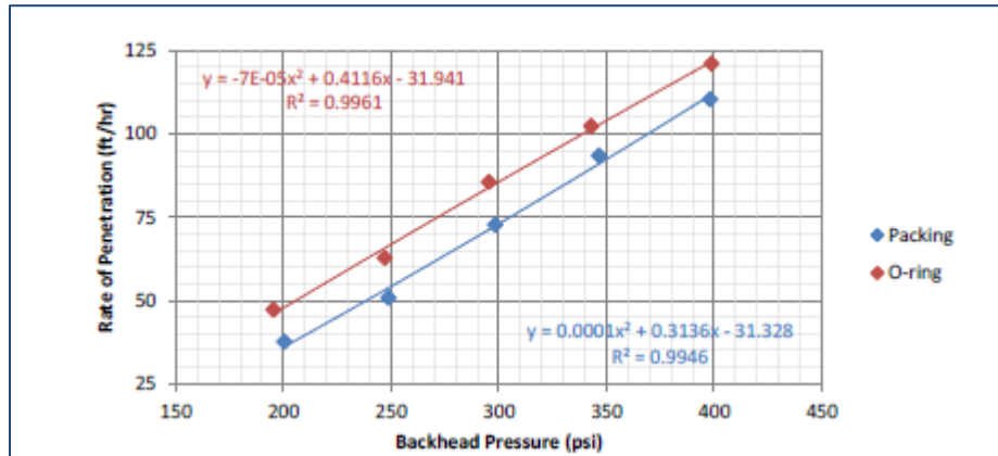
Figure 11. Rate of penetration vs. backhead pressure for preliminary baseline design
