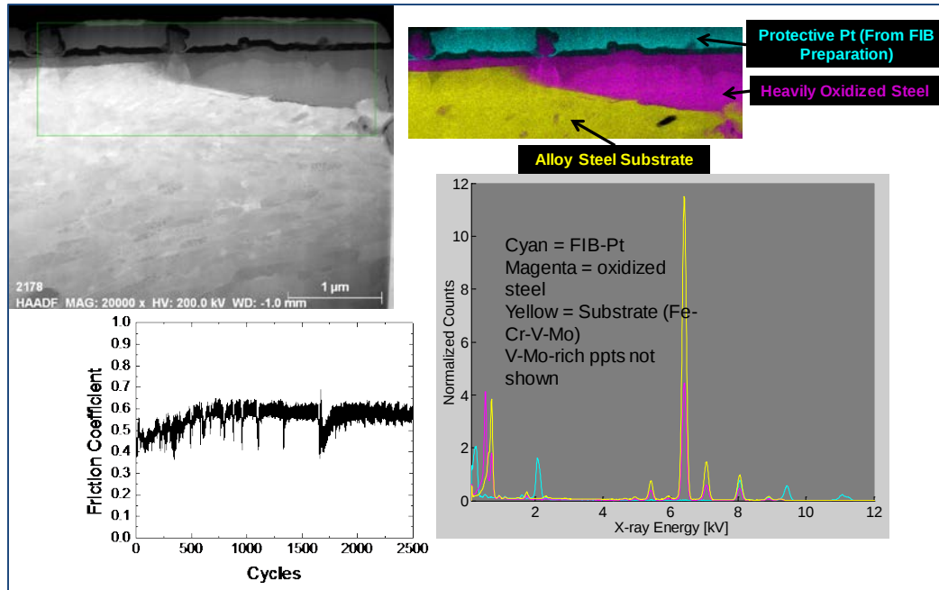
Figure 6. Results of uncoated tool steel tested at 300°C
