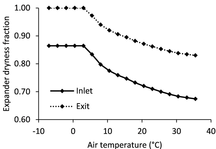
Figure 9. Expander inlet dryness fraction required for maximum net power output at off-design conditions using WORC optimised for 10.5°C air temperature, and the resultant exit dryness fraction.
