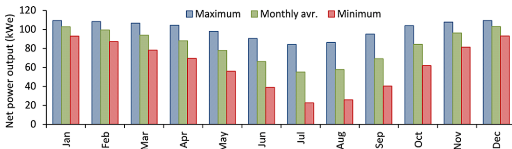
Figure 14. Maximum, minimum and time-averaged monthly net power output from WORC system optimised for 10.5°C air temperature.
