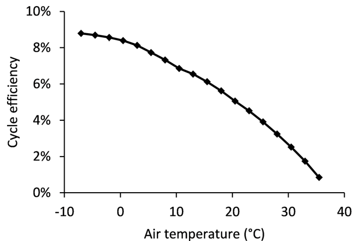
Figure 11. Cycle efficiency achieved when net power output is maximised at off-design conditions using WORC optimised for 10.5°C air temperature.
