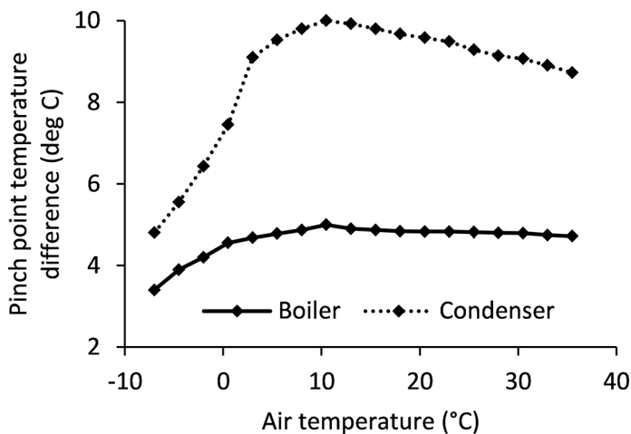
Figure 8. Boiler and condenser pinch point temperature differences required for maximum net power output at off-design conditions using WORC optimised for 10.5°C air temperature.
