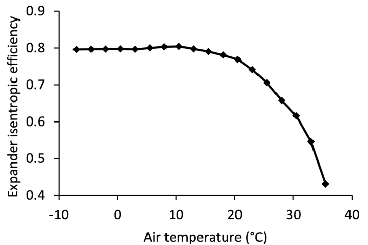
Figure 10. Expander isentropic efficiency achieved when net power output is maximised at off-design conditions using WORC optimised for 10.5°C air temperature.
