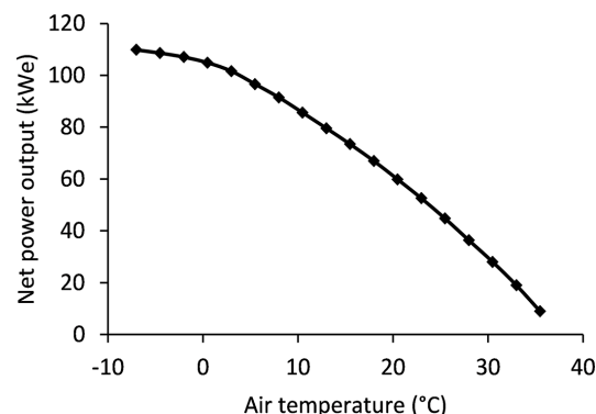
Figure 6. Maximum net power output as a function of air temperature at off-design conditions using WORC optimised for 10.5°C air temperature.
