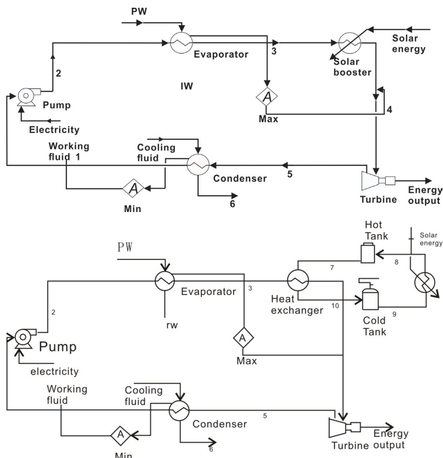
Figure 14. An ORC plant with an indirect solar heating system (Zhou et al., 2011).
