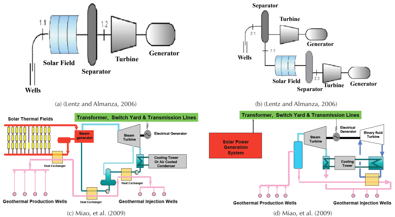
Figure 4. Different configurations of the Direct Steam Generation systems.
