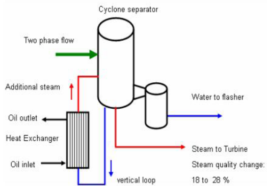
Figure 5. Heat Exchanger for heating water into a cyclonic separator (Handal et al., 2007).
