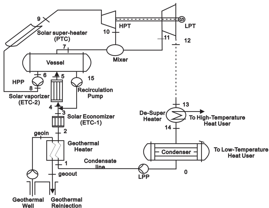
Figure 9. Dual-pressure geothermal/solar ORC layout (Tempesti et al., 2012).
