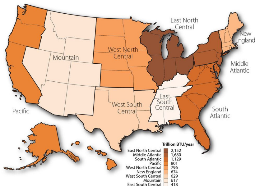
Figure 2. U.S. Heat Demand. Includes residential, commercial, and industrial heat demand. Industrial heat demand for each division was estimated from the regional data based on population. Note that this map does not include estimates of manufacturing heating/ventilating/air conditioning or any analysis of agriculture, resulting in energy totals less than the ~12 quads reported by EIA. Data source: EIA 2009, 2010, 2012. Map made by Billy Roberts NREL.
