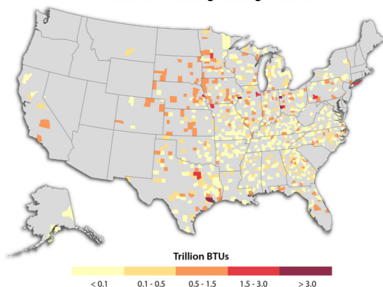
Figure 10. Industrial (manufacturing) sector thermal demand map of United States.
