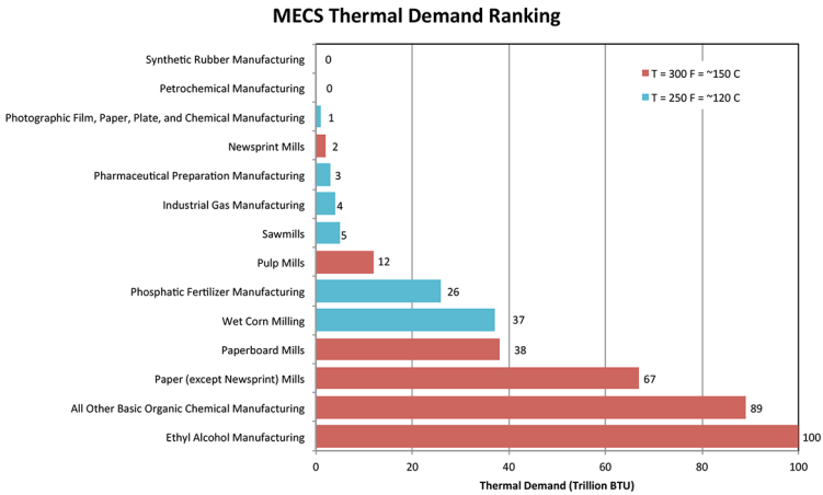
Figure 7. Thermal demand totals (trillion Btu) by industry; color coded by process steam temperature.
