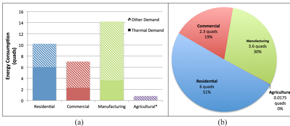
Figure 1. (a) Total energy demand in the United States by sector (~32 quads). Thermal demand is shown in solid colors in each bar. (b) Total thermal demand in the United States by sector. Source: EIA 2009, 2010, 2012.
