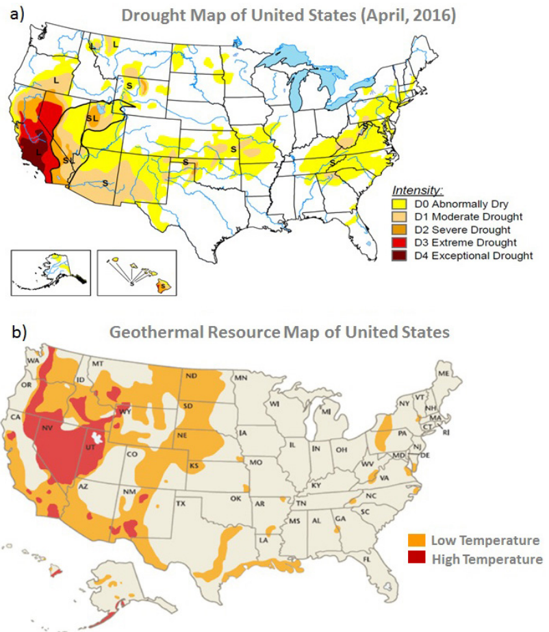
Figure 1. a) Drought map of United States in April, 2016 (NDMC, 2016) S = short-term, typically less than 6 months, L = long-term, typically greater than 6 months, b) Extent of low-temperature <100° C (orange color) geothermal resources (not including Enhanced Geothermal Systems potential) in United States (Data: OIT-GHC, 1996).
