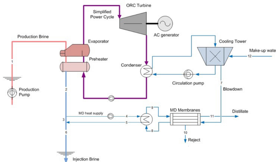
Figure 9. Conceptual process flow diagram of an MD system integrated with a water-cooled geothermal power plant.
