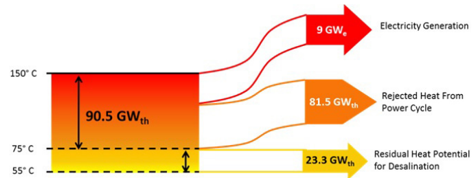
Figure 7. Residual thermal energy potential from identified medium- and high-enthalpy geothermal systems
