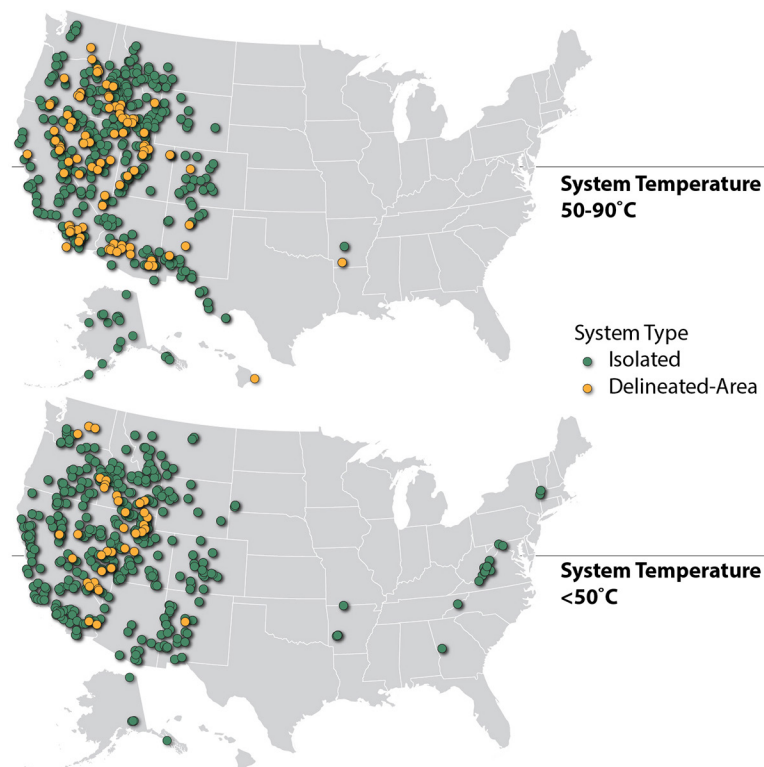
Figure 3. Distribution of low temperature hydrothermal system in United States; a) isolated and delineated-area systems having temperature between 50°C and 90°C, and b) having temperatures less than 50°C (Data Source: Reed, 1983).
