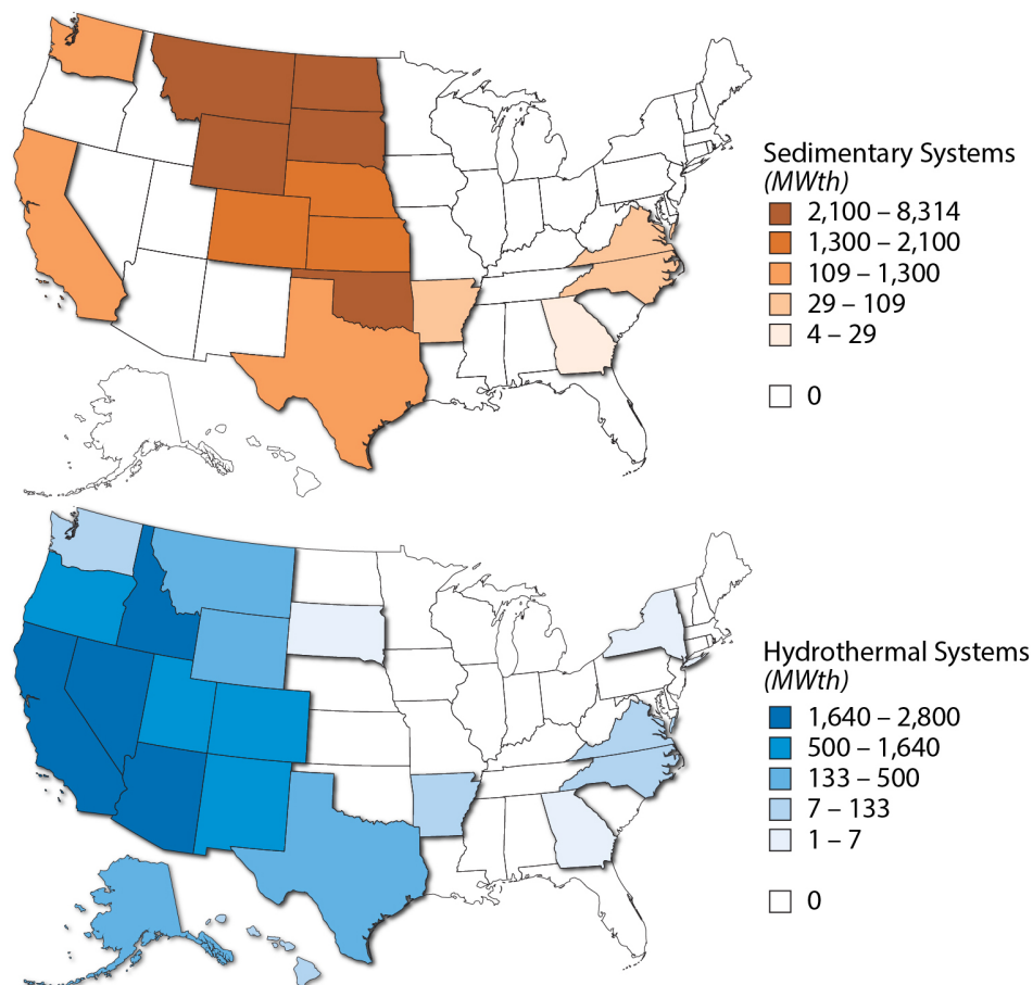
Figure 6. Distribution of estimated resource capacity of low-temperature hydrothermal and sedimentary & coastal plain systems by state (Data Source: Reed, 1983).
