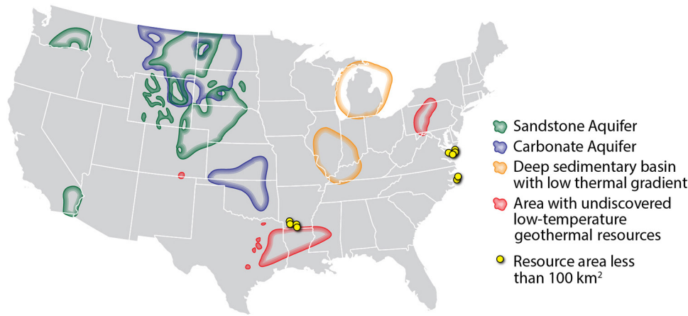
Figure 4. Distribution of low-temperature (<90°C) sedimentary geothermal systems in United States (Modified from Muffler, 1979). [Green polygons are sandstone aquifers and blue polygons are carbonate aquifers with sandstones having reservoir temperature below 90 °C and above the minimum temperature criterion. Red polygons are areas with undiscovered resources in coastal plains with permeable unknown reservoir rocks overlain by impermeable shale formation having low temperature geothermal potential. Orange polygons are the Deep Sedimentary systems (>2 km) with low thermal gradient (<25°C) and unknown reservoir type. Yellow points represent small scale (<100 km²) coastal plain systems with low-temperature resource potential.]
