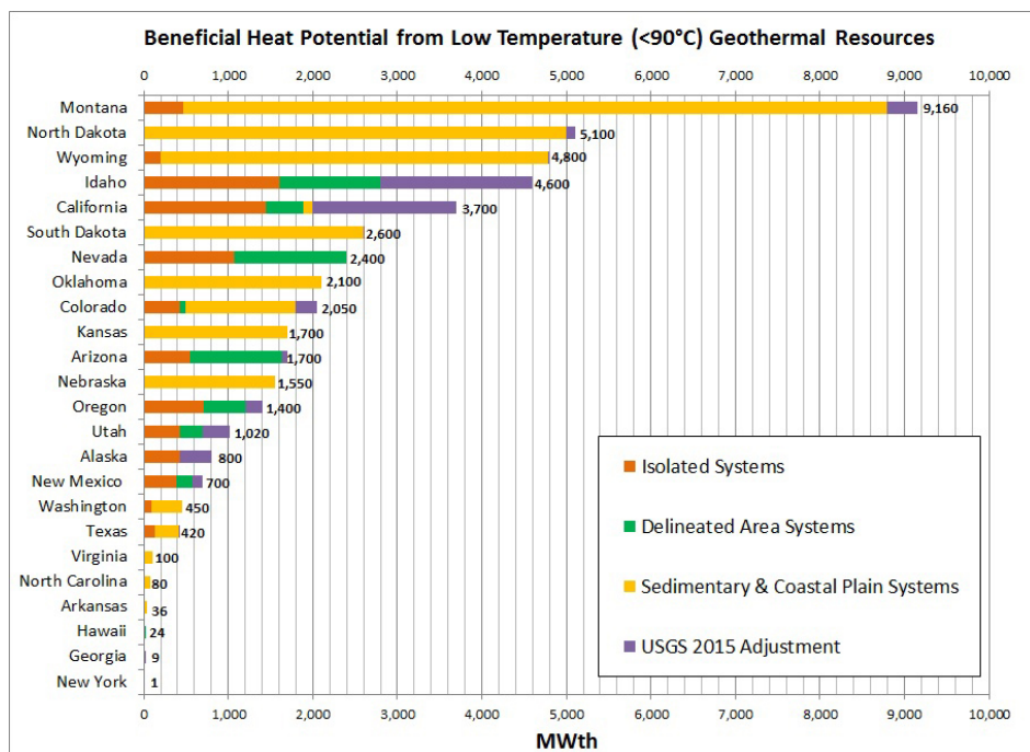
Figure 5. Beneficial geothermal heat potential by state originating from isolated, delineated and sedimentary systems (Original data source: Reed, 1983; Williams et al, 2015) Note: The USGS 2015 adjustment did not breakdown the additional heat potential by system category.
