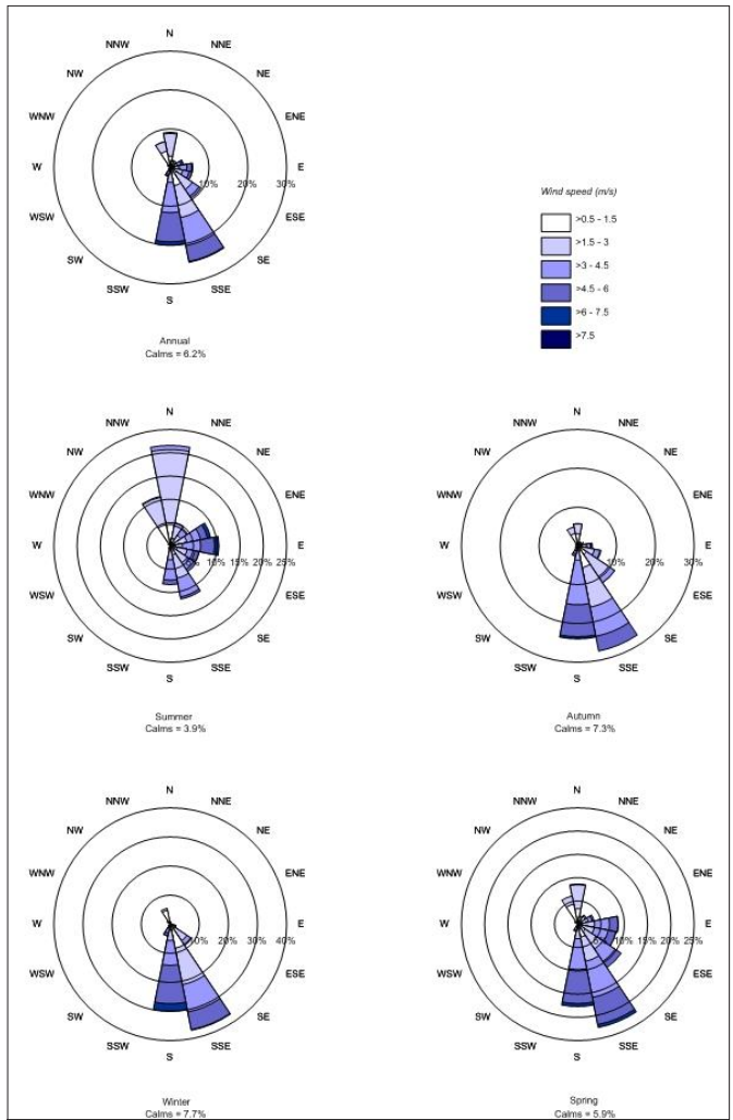
Figure 3. Olkaria wind roses derived from Calmet Model at 10m above ground level.
