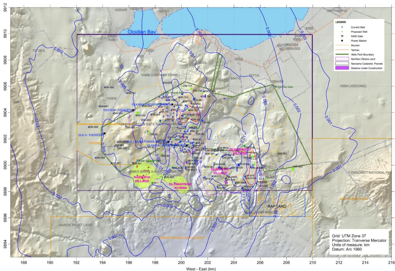
Figure 12. Predicted annual average hydrogen sulphide concentrations for Case 3 operations (in ppm).
