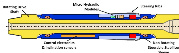
Figure 4. Main components of a RSS push-the-bit system (Source: Baker Hughes).
