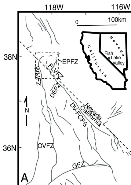
Figure 1A. Location of Fish Lake Valley within the regional-scale tectonic regime (modified from Reheis and Sawyer, 1997). Dashed polygon shows extent of figure 1B.
