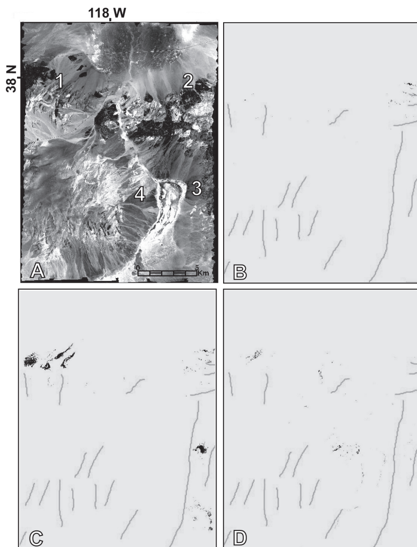
Figure 2A. Georeferenced spatial extent of the 2003 HyMap survey in greyscale. White numbers equal exploration targets of interest as delineated from first-tier indices algorithms. B, C and D are specific mineral group distribution images plotted with local faulting taken from Reheis and Sawyer, 1997. B. Kaolinite-rich areas C. Mica-rich areas D. Carbonate/chlorite-rich areas.
