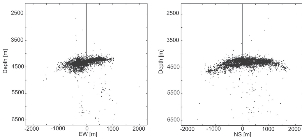
Figure 6. Collapsed seismic location
