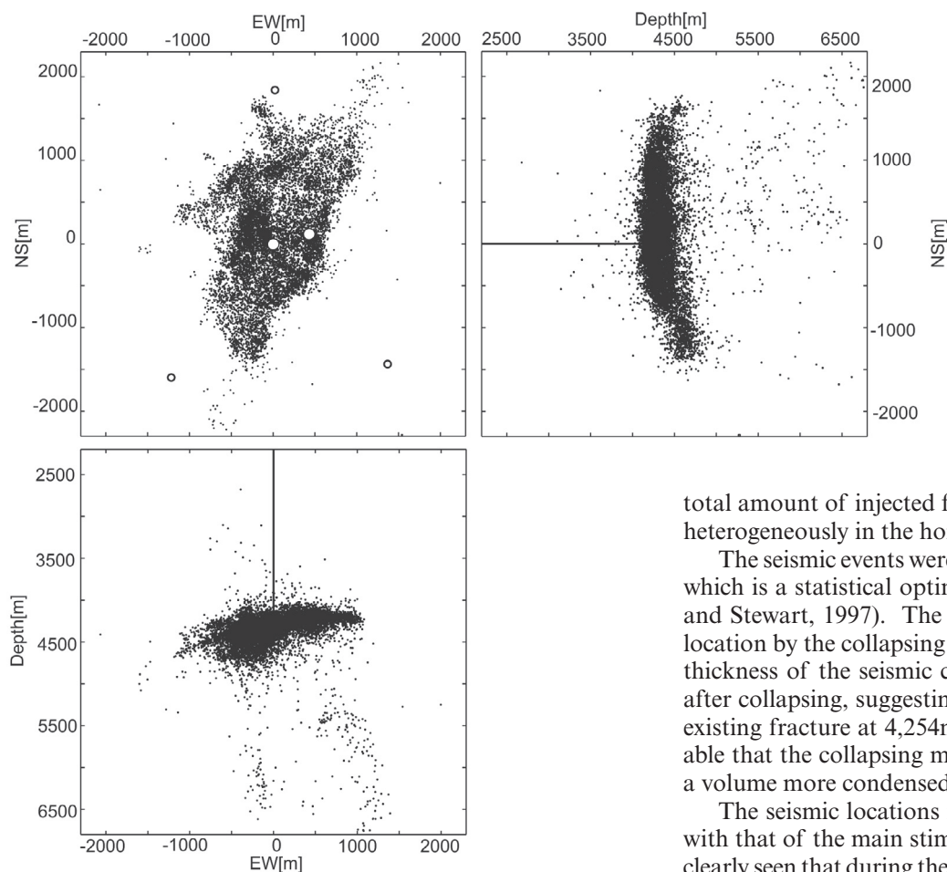
Figure 3. 3D distribution of the seismic location for all the tests and stimulations.
