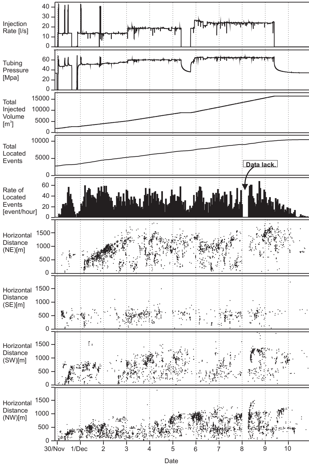
Figure 5. Source migration in the first 11 day of the 1 st stimulation.
