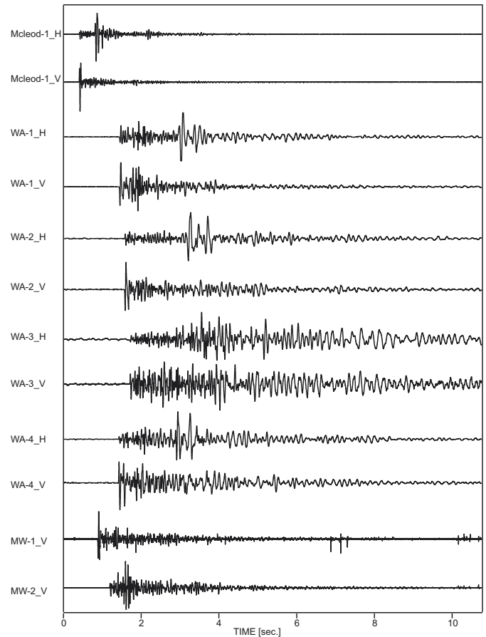
Figure 2. Typical seismic trace detected by the stations.
