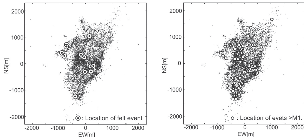
Figure 4. Location of events with larger energy.
