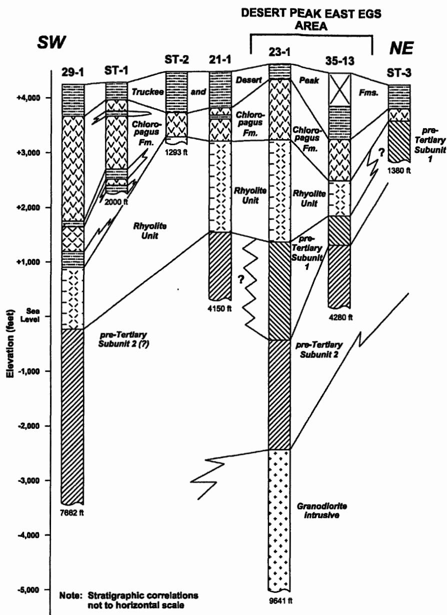
Figure 4. Stratigraphic correlations across the Hot Springs Mountains and the Desert Peak East EGS project area (stratigraphy of wells within the hydrothermal portion of the Desert Peak field from Benoit and others, 1982). Structural interpretations have not been attempted nor are implied.
