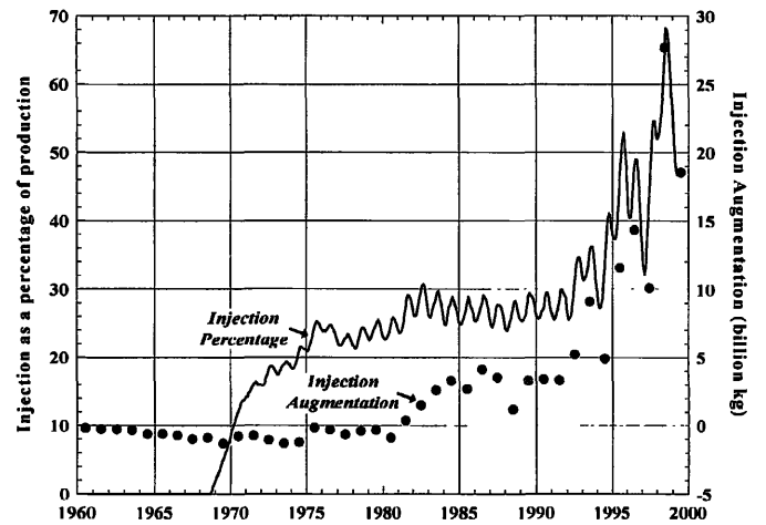
Figure 7. Injection History at The Geysers.
