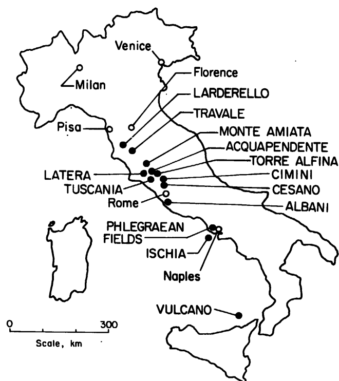
Fig. 5 Geothermal plant sites/prospects in Italy.
