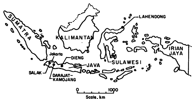
Fig. 9 Geothermal plant sites/prospects in Indonesia
