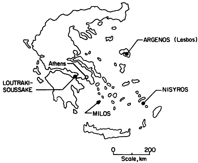
Fig. 16 Geothermal plant sites/prospects in Greece.
