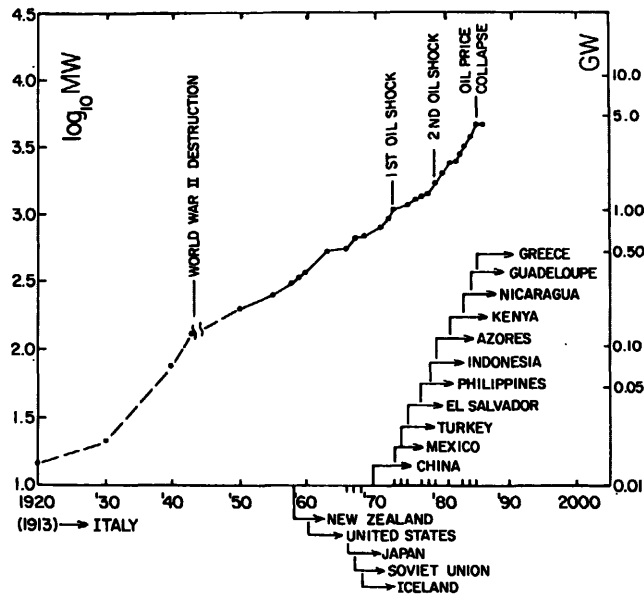
Fig. 1 Growth pattern for geothermal power: installed megawatts versus year.
