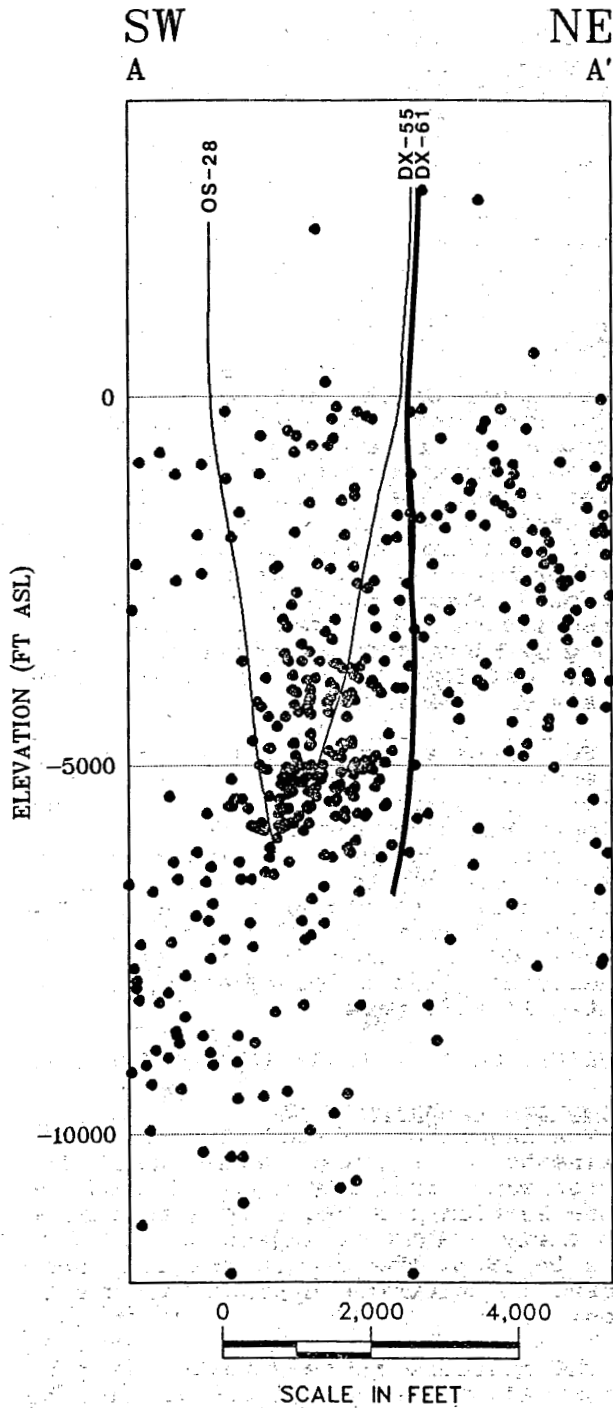
Figure 5. MEQ cross-section A-A', DX-61 area, 9/86 - 12/86, immediately after startup of injection into DX-61 (bold well course). Note how the MEQ plumes dip SW from DX-61 towards producing wells OS-28 and DX-55. Figure 2 shows pertinent temporal correlations. Cross-section width is 3,000 ft; trace is shown on Figure 4.
