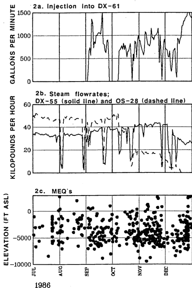
Figure 2. Time history (7/86 - 12/86) of injection into DX-61 (location in Figure 1), steam flowrates at DX-55 and OS-28, and MEQ depths within a 4,000 ft square centered on DX-61. After the onset of injection on 9/2, the two producers experienced temporary flowrate increases and MEQ activity deeper than 3,000 ft subsea more than tripled.
