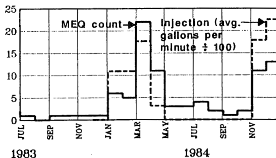
Figure 3. Time history of injection into GDC-18 (location in Figure 1) in average gallons per minute (GPM) and monthly count of MEQ's deeper than 3000 ft subsea within a 2000 ft square centered on GDC-18. MEQ count is based on USGS data.
