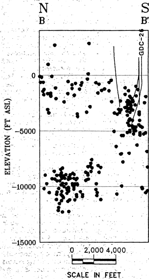
Figure 6. MEQ cross-section B-B', GDC-26 area, 11/88- 8/89, coda magnitudes > 0.7. All four injection wells shown were active during this time span. Note how the deep MEQ plumes spread north and south from the injectors. Cross-section width is 3,000 ft; trace is shown on Figure 4.
