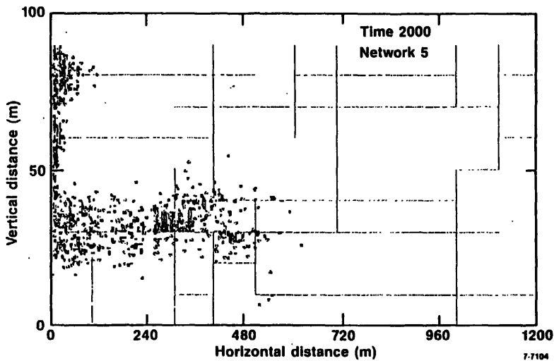
Figure 2. Extent of cooling between injection well (left) and production well (right) in a fractured reservoir after 2000 days of injection.
