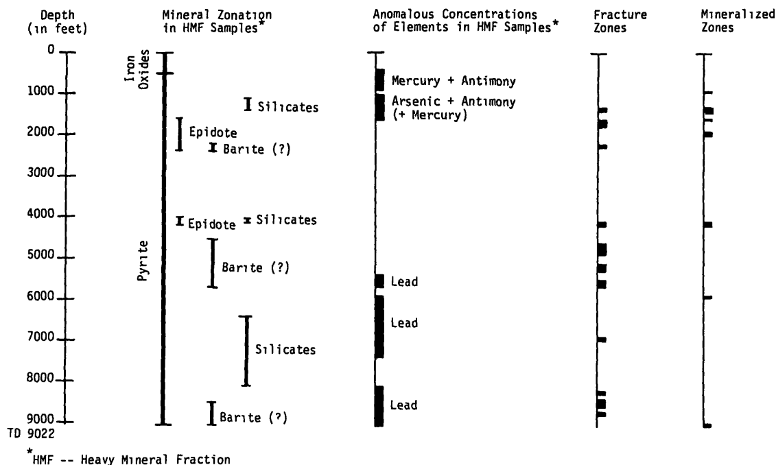
Figure 4. Composite of logs for DF 45-14 indicating selected physical parameters, mineral occurrences and anomalous element concentrations in heavy mineral fraction samples.
