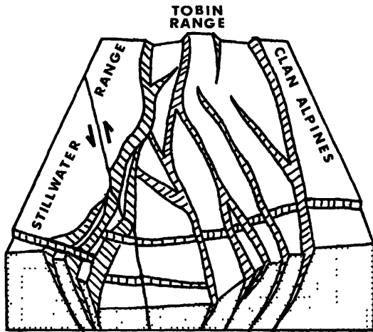
Figure 2. Structural model of northern Dixie Valley, with alluvium removed and bedrock surfaces restored (from Whitney, 1980).
